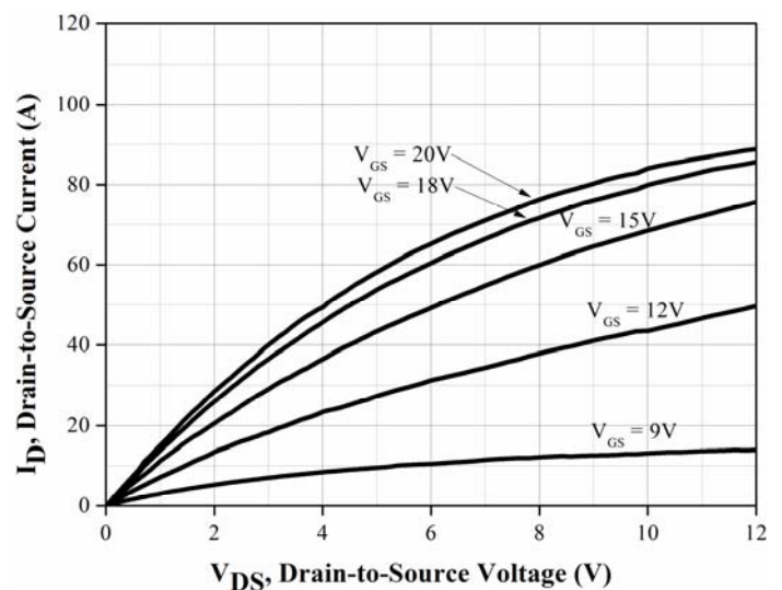
Figure2. Output Characteristics Tj = 25℃
