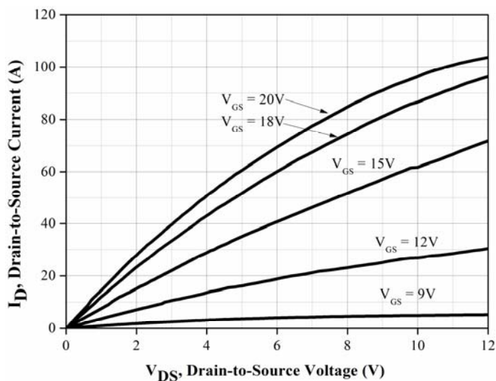
Figure 1. Output Characteristics Tj = -55℃
