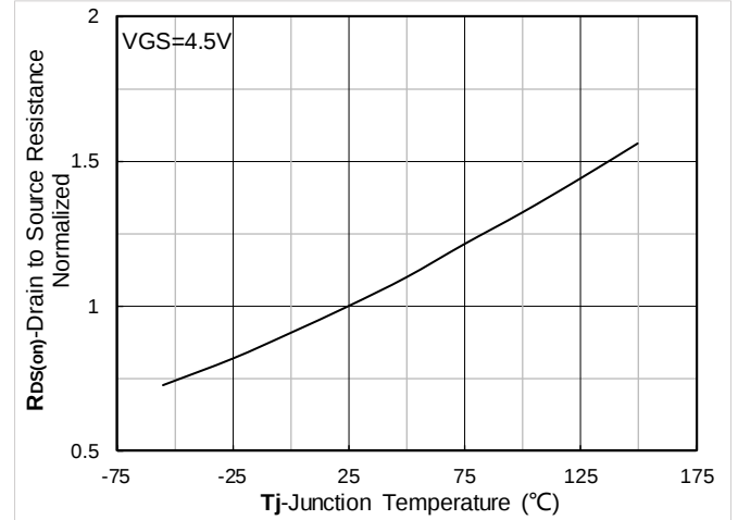
Figure 6. Normalized On-Resistance
