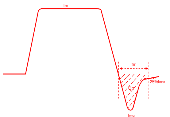
Figure C. Diode Recovery Test Circuit & Waveform
