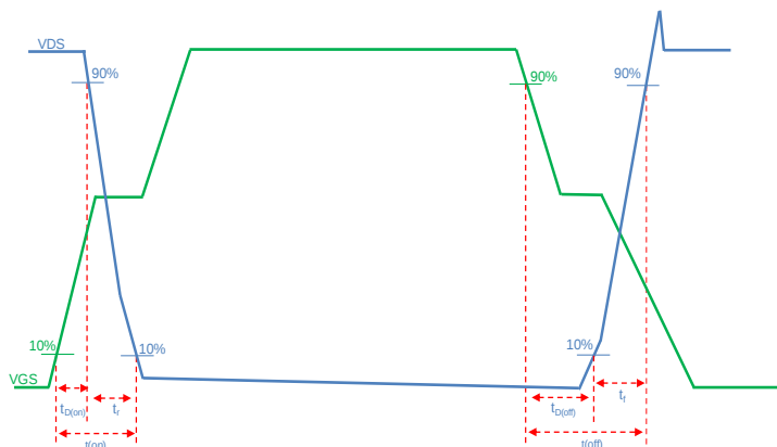
Figure B. Resistive Switching Test Circuit & Waveform
